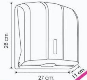
Z Folded Paper Towel Dispenser Z Katlı Kağıt Havlu Dispenseri
