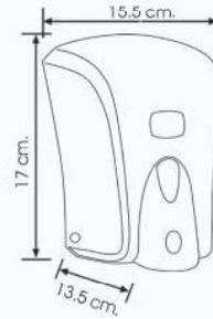
Medical Foam Dispenser With Cartridge 800 ml. Kartuşlu Medikal Köpük Dispenseri
