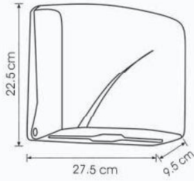
Z Folded Paper Towel Dispenser Z Katlı Kağıt Havlu Dispenserli
